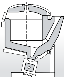
Channel furnaces \ Horno de canal
